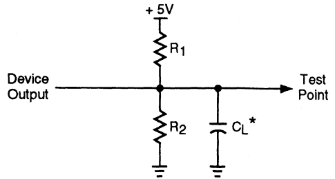
Figure 2. Test Load
