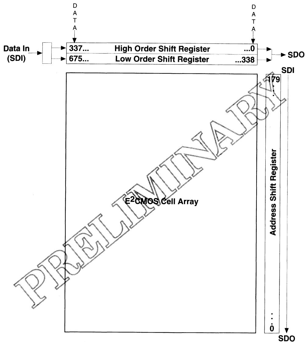
Figure 7. ispLSI 3256 Shift Register Layout
