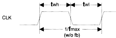
Clock Width
