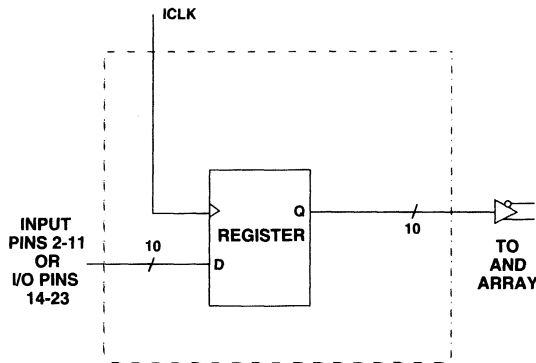
Registered Input
