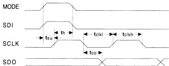
Figure 5. Shift Register Timing
