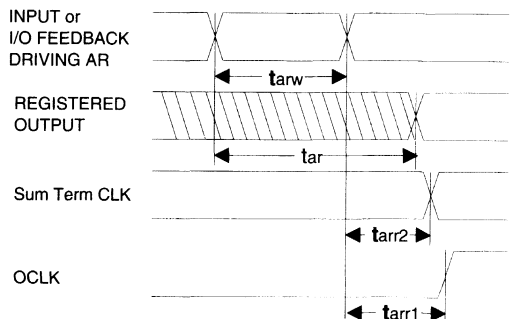
Asynchronous Reset
