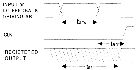
Synchronous Preset
