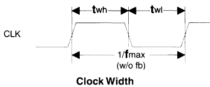
Clock Width
