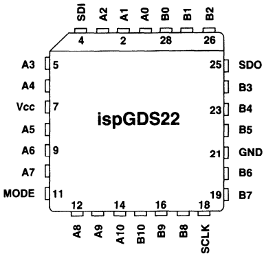
28-Pin PLCC
