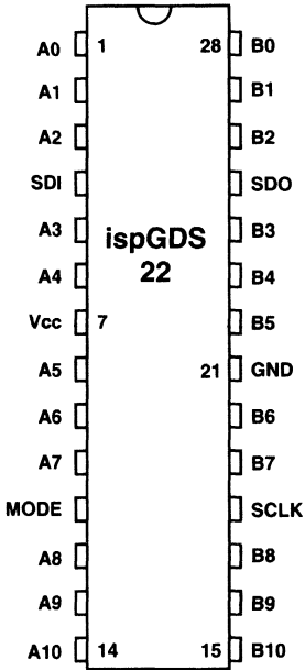
28-Pin DIP
