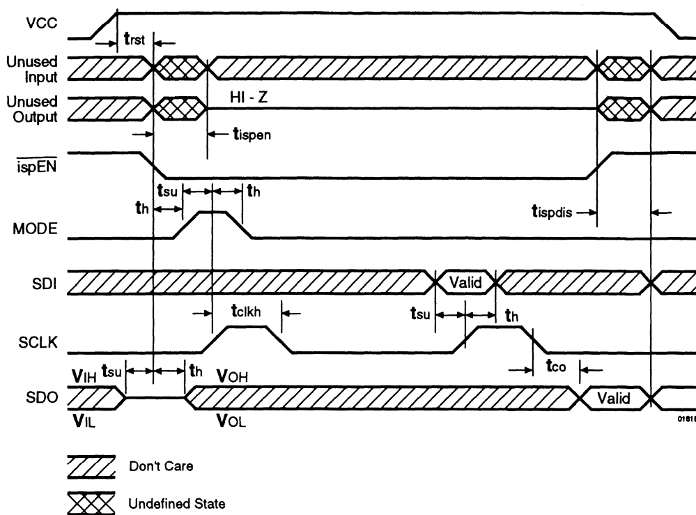
Figure 6. Timing Waveforms for In-System Programming (ispLSI 1048)
