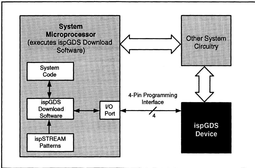
Figure 1 — In-System Programming Using ispGDS Download Software
