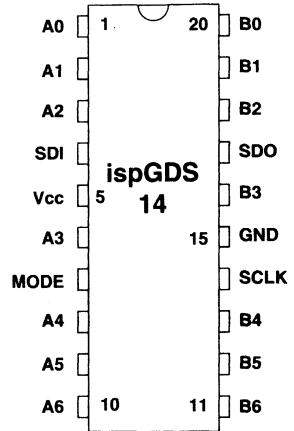
20-Pin DIP
