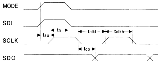
Figure 6. Shift Register Timing
