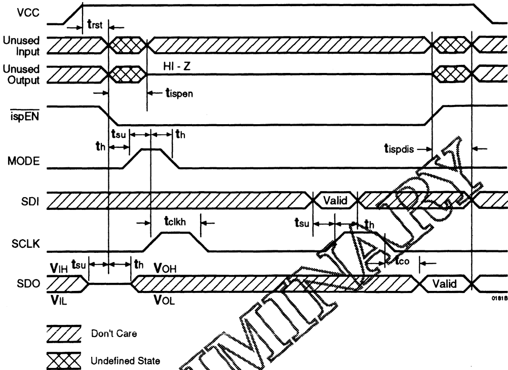
Figure 5. Timing Waveform for In-System Programming
