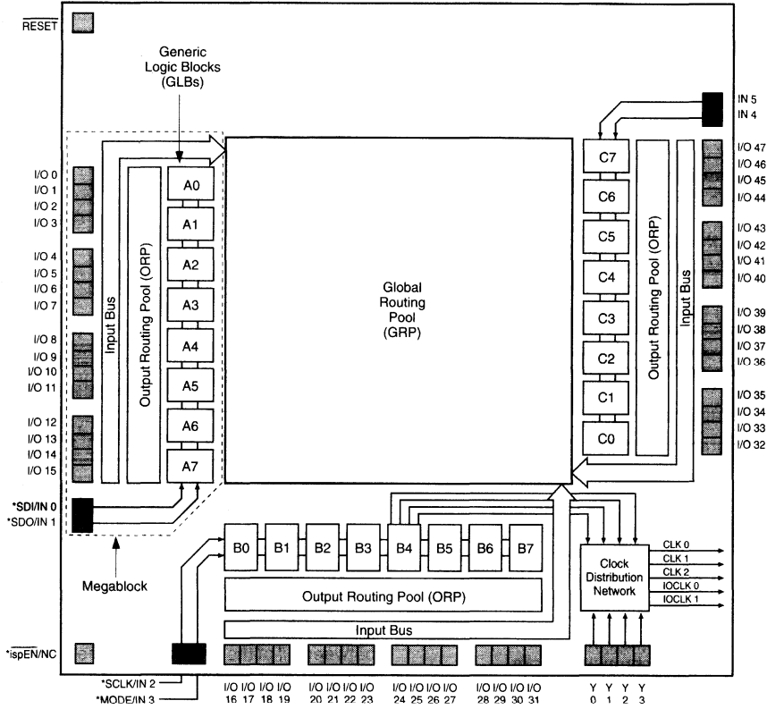
Figure 1. pLSI and ispLSI 1024 Functional Block Diagram
