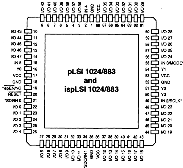
pLSI and ispLSI 1024 68-Pin JLCC Pinout Diagram
