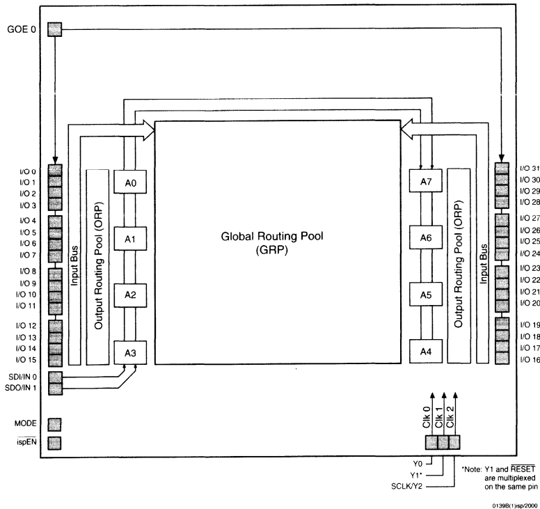
Figure 1. pLSI 2032 Functional Block Diagram
