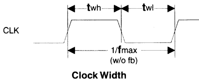
Clock Width
