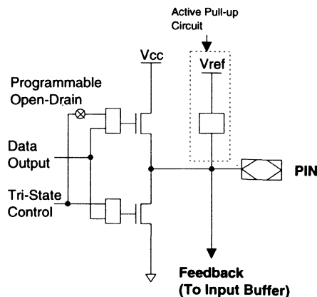
Typical Output
