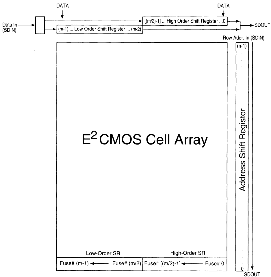
Figure 7. ispLSI Device to Fuse Map Translation
