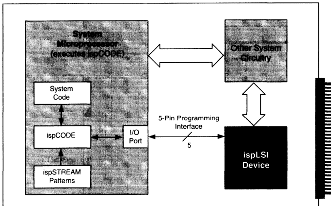
Figure 12. Configuring an ispLSI Device from an On-Board Microprocessor
