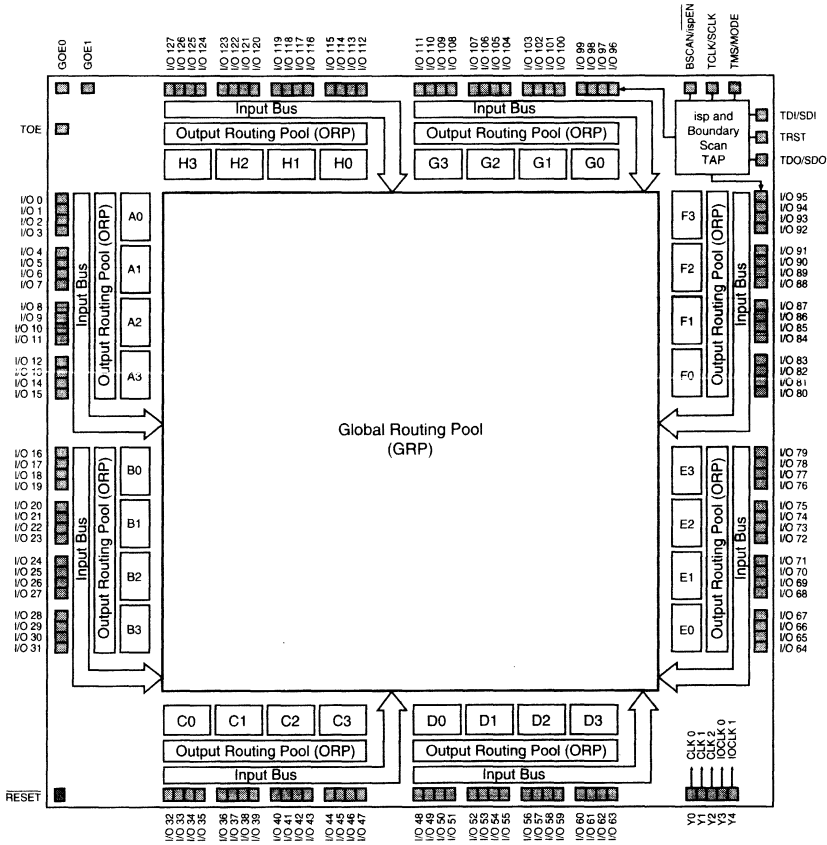
Figure 1. ispLSI 3256 Functional Block Diagram
