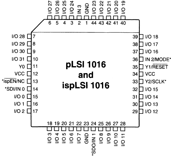
pLSI and ispLSI 1016 44-Pin PLCC Pinout Diagram
