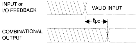
Combinatorial Output
