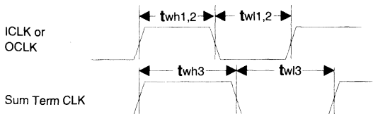
Clock Width
