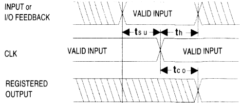
Registered Output
