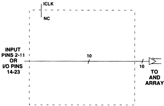
Asynchronous Input
