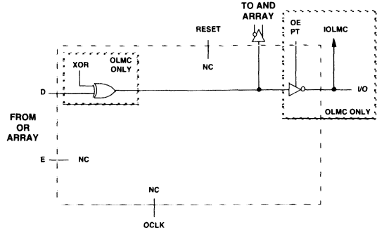
Combinatorial
