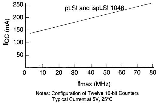
Figure 3. Typical Device Power Consumption vs fmax
