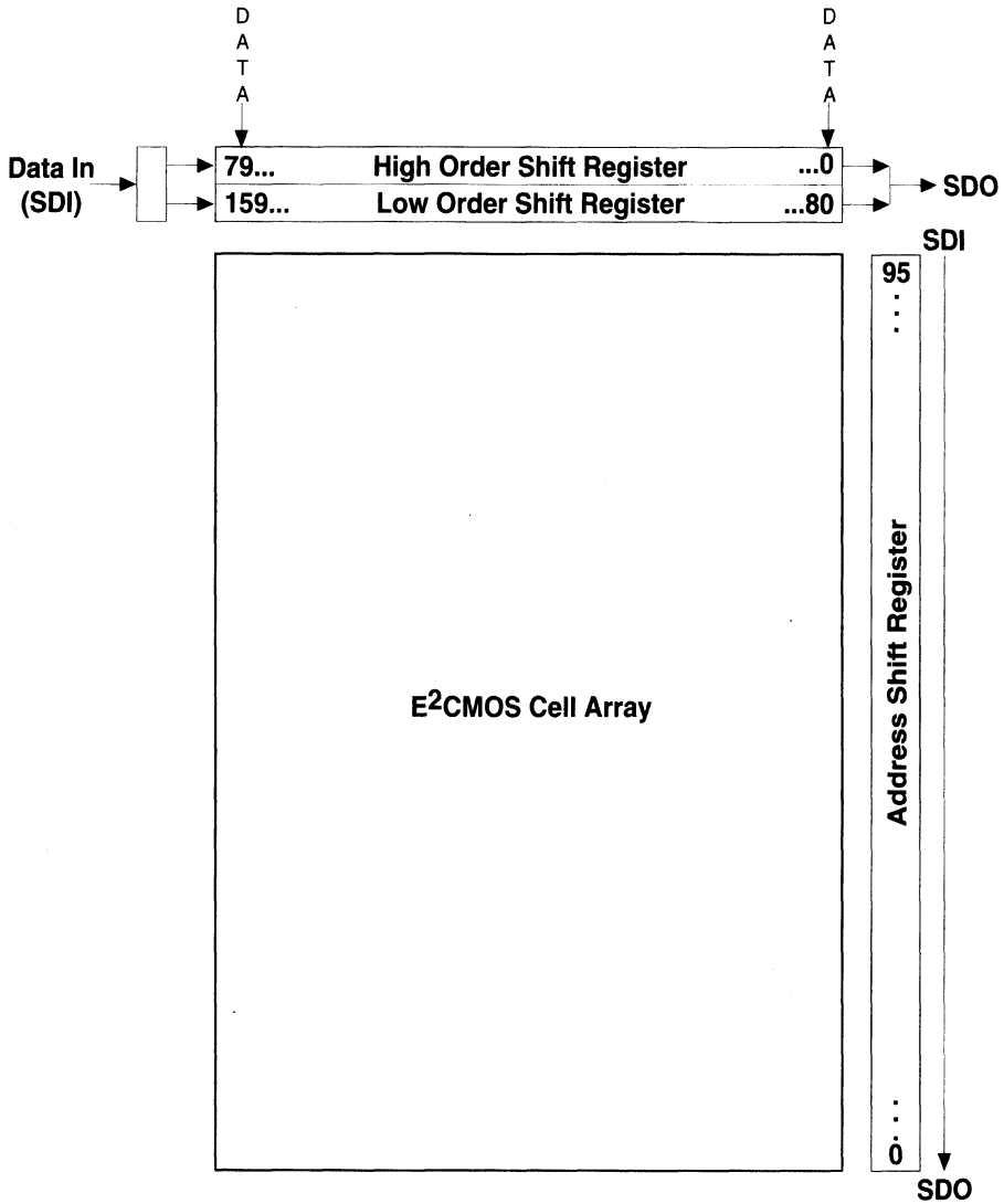
Figure 8. ispLSI 1016 Shift Register Layout
