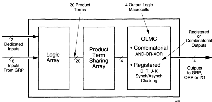
Figure 3. pLSI and ispLSI 3000 Family "Twin GLB"
