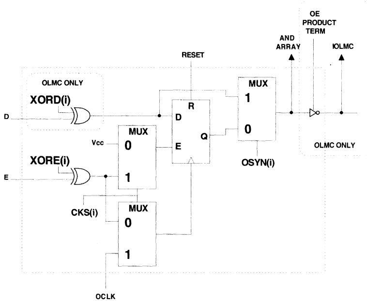
OLMC/BLMC Generic Logic Block Diagram
