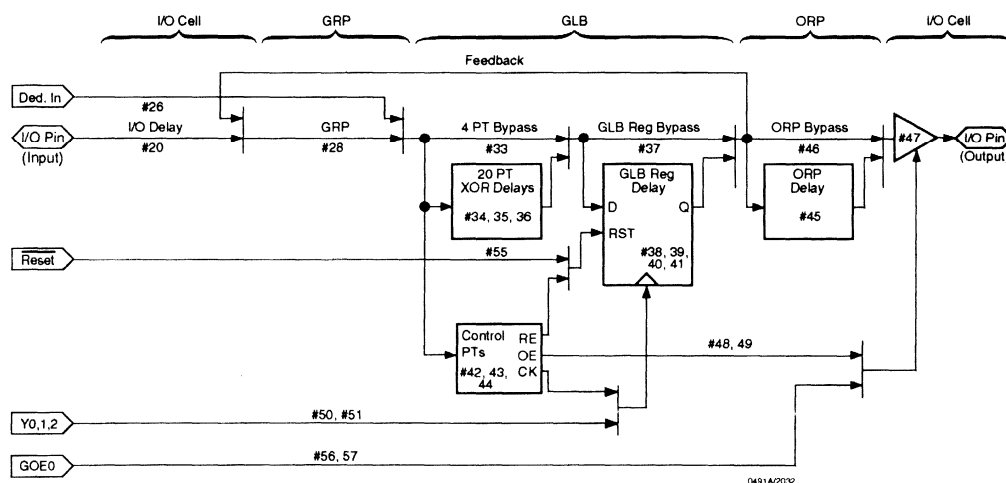
Figure 8. pLSI and ispLSI 2032 Timing Model
