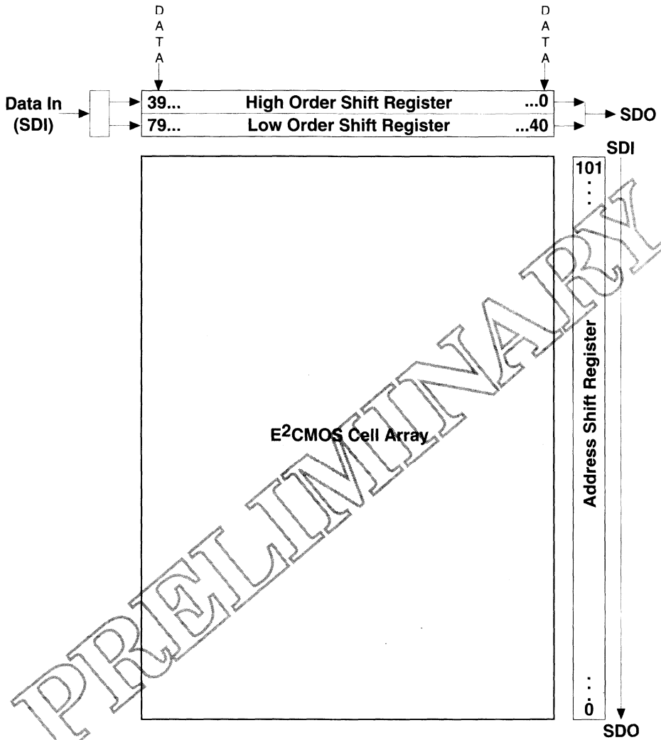
Figure 7. ispLSI 2032 Shift Register Layout
