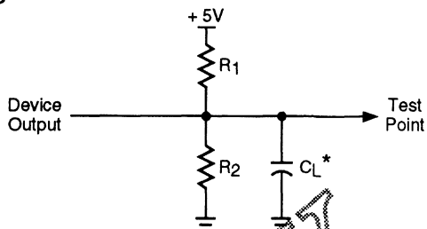
Figure 2. Test Load
