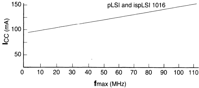
Figure 3. Typical Device Power Consumption vs fmax
