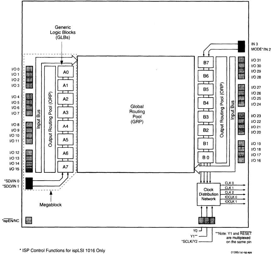
Figure 1. pLSI and ispLSI 1016 Functional Block Diagram
