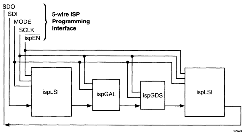
Figure 5. ISP Programming Interface
