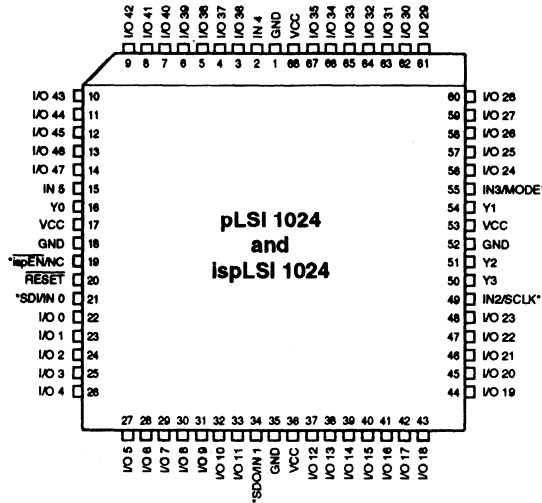
pLSI and ispLSI 1024 68-Pin PLCC Pinout Diagram
