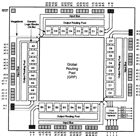
Figure 1. pLSI 1032 Functional Block Diagram
