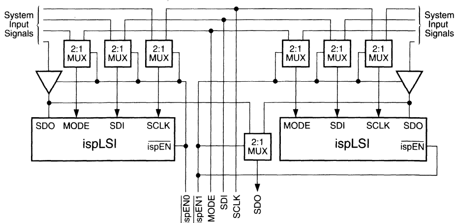
Figure 2. The Scan and Multiplex Programming Mode
