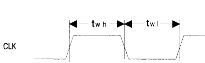
Clock Width
