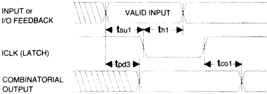
Latched Input
