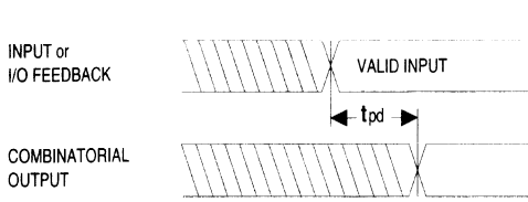
Combinatorial Output
