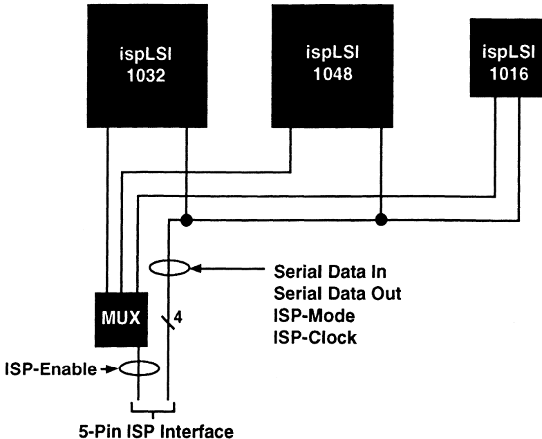
Figure 1. ispLSI Programming Interface
