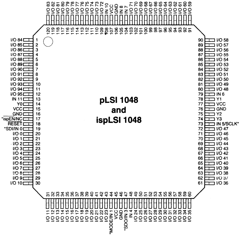
pLSI and ispLSI 1048 120-Pin PQFP Pinout Diagram
