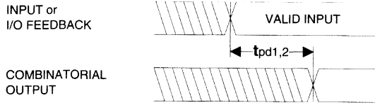
Combinatorial Output
