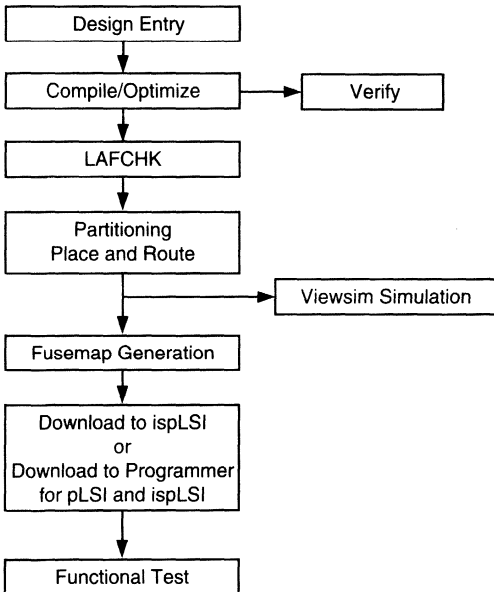
Figure 2c. pDS+ LOG/iC Design Flow
