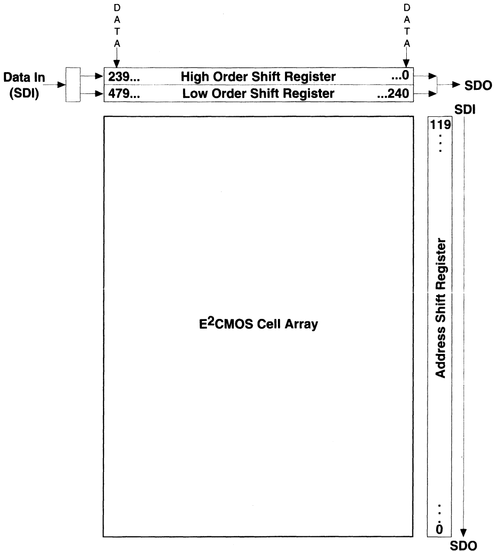
Figure 8. ispLSI 1048 Shift Register Layout
