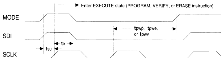
Figure 6. Program, Verify, & Erase Timing
