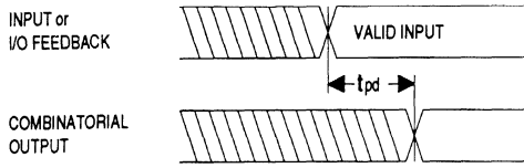
Combinatorial Output
