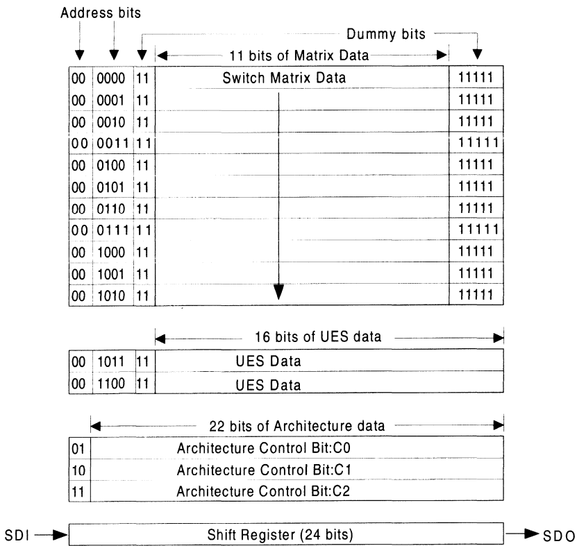
Figure 7. ispGDS Architecture
