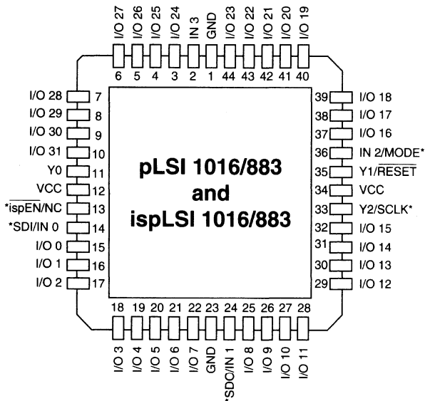
pLSI and ispLSI 1016 44-Pin JLCC Pinout Diagram
