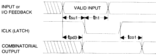
Latched Input
