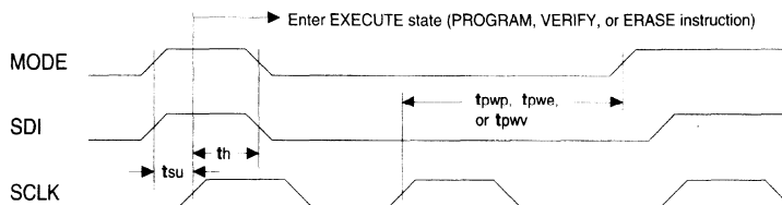
Figure 7. Program, Verify, & Erase Timing
