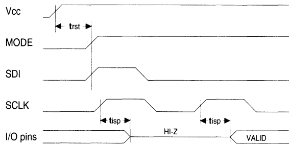
Figure 4. Programming Mode Timing
