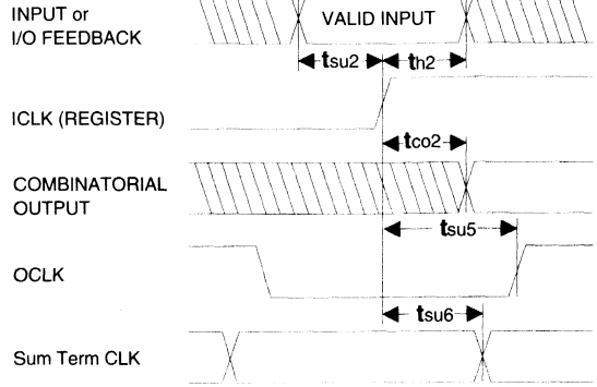
Registered Input
