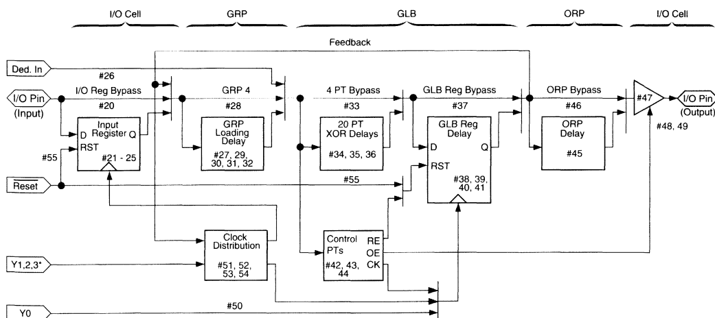
Figure 14. pLSI and ispLSI Timing Model 1
