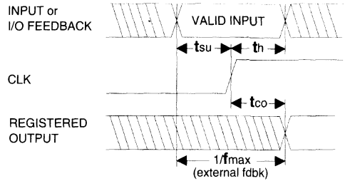
Registered Output
