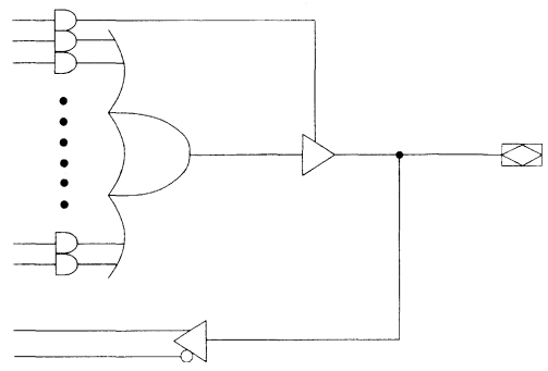
ACTIVE HIGH
