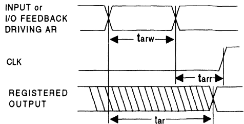
Asynchronous Reset
