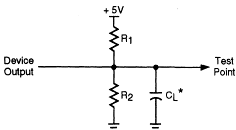
Figure 2. Test Load
